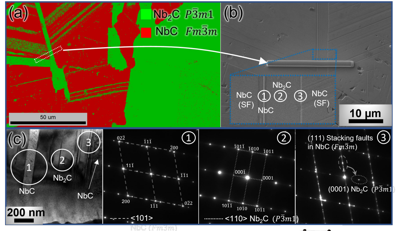
Figure: (a) Phase map that reveals laths of Nb 2 C (green) forming in NbC (red) (b) Site specific sample extraction of a lath region (c) electron microscopy image revealing nanoscale laths with 1, 2, and 3 being electron scattering patterns confirming the new C6 structure. More details at doi.org/10.1007/s11837-023-06084-y
