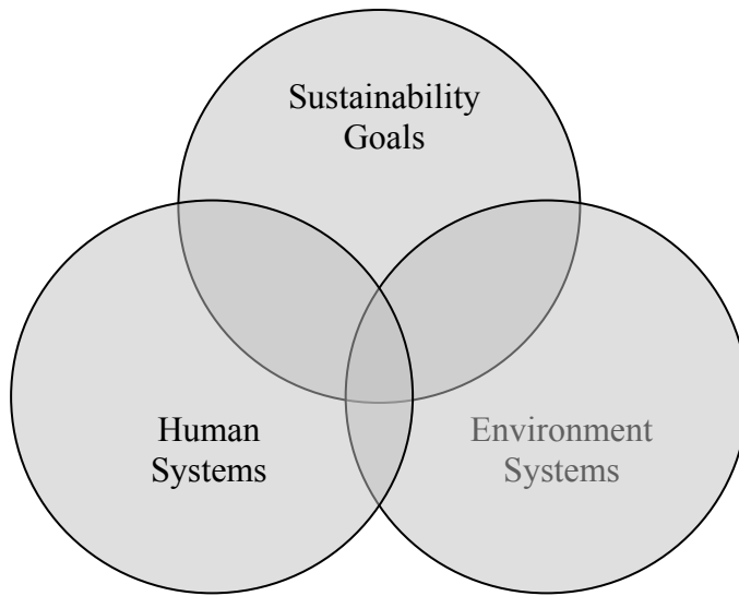
Figure 3: The domain of sustainability science
